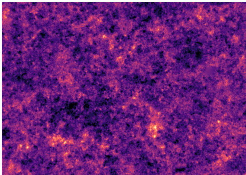
Dark matter distribution
