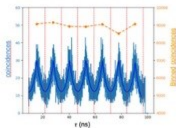
Photon antibunching of rhodamine dyes
