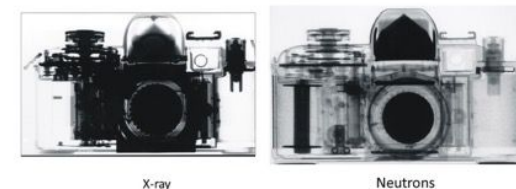
Comparison of X-ray and Neutron Radiographs
